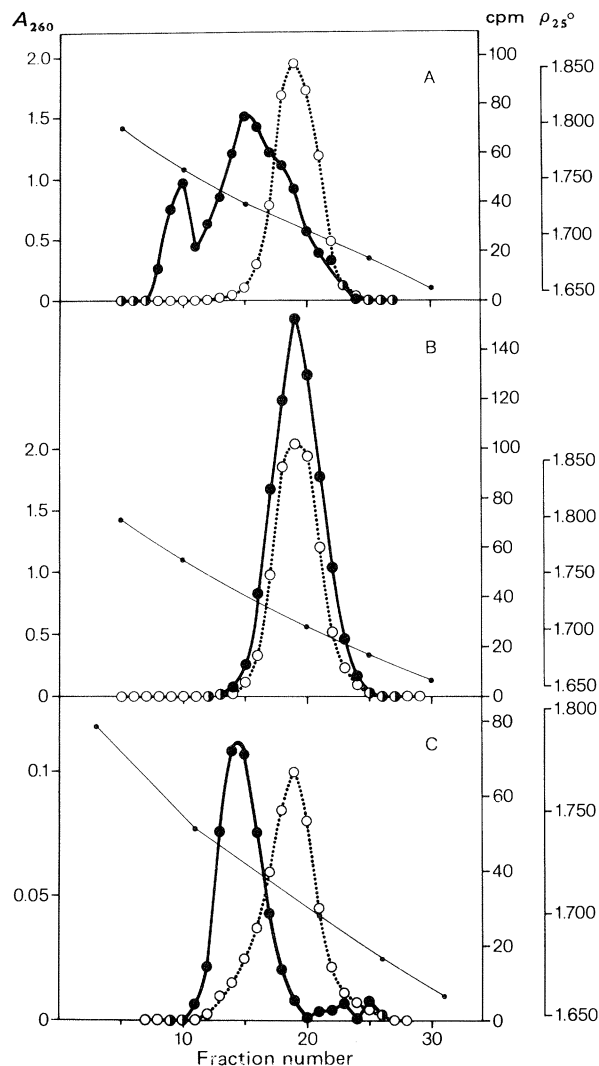
FIG. 2. Preparative R-loop formation. EcoRI -digested embryonic DNA pre-fractionated by agarose gel electrophoresis for V_{\lambda} gene sequences was incubated in the presence (A) and absence (B) of HOPC 2020 \lambda chain mRNA and centrifuged in CsCl as described in Materials and Methods . Fractions 12 to 16 shown in A and another tube which showed profiles nearly identical to A were pooled and recentrifuged (C). \circ \cdots \circ , A_{260} ; \bullet \cdots \bullet , DNA-RNA hybrid; \bullet \cdots \bullet , buoyant density.
