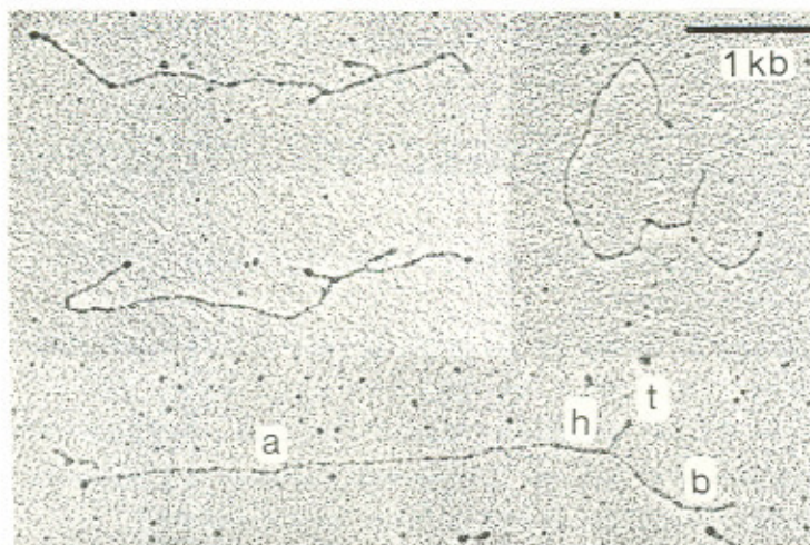
Figure 4: Hybrid molecules made by annealing cDNA to denatured Ig 13 DNA. The structure consists of two single-stranded arms (a,b), the double-stranded homology region (h) and a single-stranded tail (t). The different parts of the molecules were measured, using as internal standards DNAs of phages fd and PM2.
