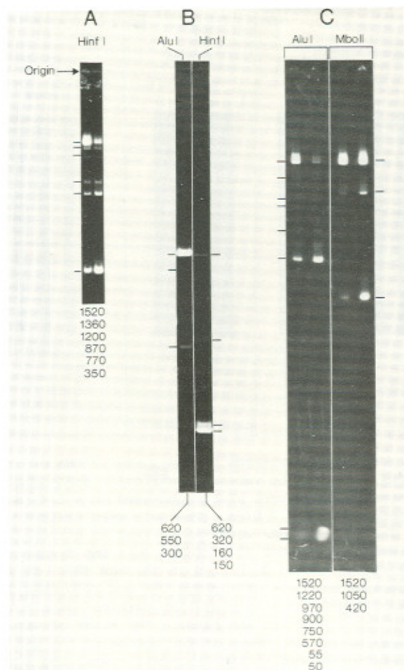
Figure 7: Autoradiogram of 1.52 kb Hae III B fragments and 0.62 kb Hind III fragments partially digested with various restriction endonucleases. (A): the end-labeled 1.52 kb Hae III DNA fragment (760 cpm) was partially digested with Hinf I and fractionated by electrophoresis through a 3.5% acrylamide gel for 11 h at a potential of 3 V/cm. (B): the terminally - labeled 0.62 kb Hind III fragment (4700 cpm) was partially digested with the restriction enzymes indicated and electrophoresed as described in Figure 6A. The autoradiogram shown was allowed to develop for 12 h. (C): the end-labeled 1.52 kb Hae III fragment was partially digested with the restriction enzymes indicated and analyzed as described in the legend to Figure 6A. SV40 DNA digested with Hind III was terminally-labeled with polynucleotide kinase and used as a migration marker (data not shown). The autoradiogram shown was developed for 3 days. In (A), (B) and (C), the sizes of fragments (in base pairs) are shown at the bottom. The lines beside the lanes indicate DNA bands.
