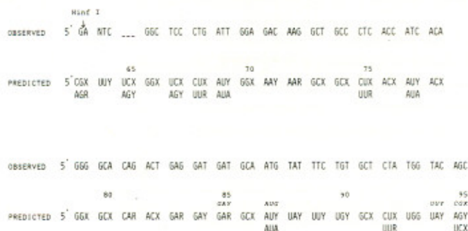
Figure 10: Partial nucleotide sequence of the left half of the Hinf 330 base pair fragment. The observed nucleotide sequence (Figure 9A) is shown in comparison with that predicted from the amino acid sequence of a V_{\lambda II} region (MOPC 315 \lambda chain), which is identical with that of V_{\lambda I} (MOPC 104E \lambda chain) except for positions 85, 87, 94 and 95. Nucleotide sequences predicted from MOPC 315 \lambda chain at these positions are shown in italics. Positions 94 and 95 are within a hypervariable region. X,N: any one of the four bases. R: purine. Y: pyrimidine.
