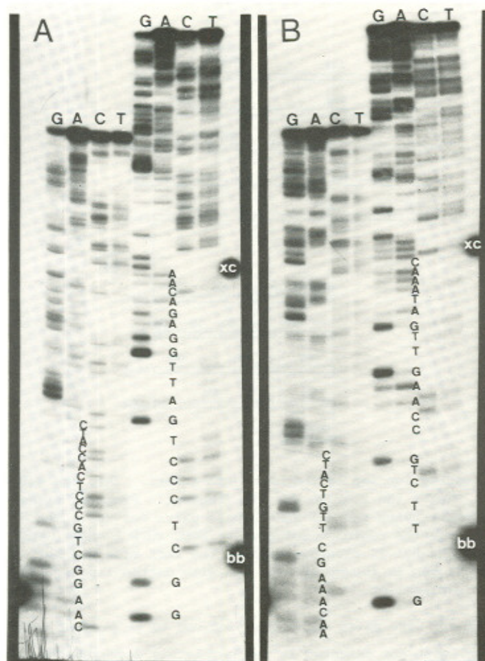
Figure 9: Sequencing gels of the Hinf 330 base pair fragment. The fragment was end-labeled with polynucleotide kinase, cleaved with Mbo II and the resulting fragments, A (left) and B (right) were separated by gel electrophoresis. The two fragments were treated according to Maxam and Gilbert (14) in four separate reactions cleaving the sequence at G>A, A>G, C>T and C+T. The gels contained 20% acrylamide and 7 M urea and were run at 800-1000 volts. The positions of the marker dyes, xylene cyanol and bromphenol blue, are indicated. Panel A shows a sequencing gel of the left fragment, Mbo II, containing sequences homologous to \lambda chain mRNA. Panel B shows a sequencing gel of the right end of the Hinf fragment. Note that in this gel the bands in the pyrimidine cleavage reactions are slightly delayed relative to the purine cleavage bands, probably due to incomplete elimination of the piperidine from the samples applied to the gel.
