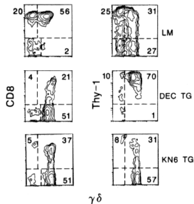
FIGURE 9. Comparison between CD8 and Thy-1 expression by IEL from DEC and KN6 transgenic mice and age-matched nontransgenic mouse. IEL from V_{\gamma 4}V_{\delta 5} transgenic ( bottom ), V_{\gamma 5}V_{\delta 1} transgenic ( middle ), and nontransgenic ( top ) 8-wk-old mice were stained with 3A10 (anti- \gamma/\delta ) mAb (FITC conjugated) and either CD8 ( left ) or Thy-1.2 ( right ) mAbs (biotinylated, streptavidin-phycoerythrin). Indicated is the percent of cells in each quadrant.
