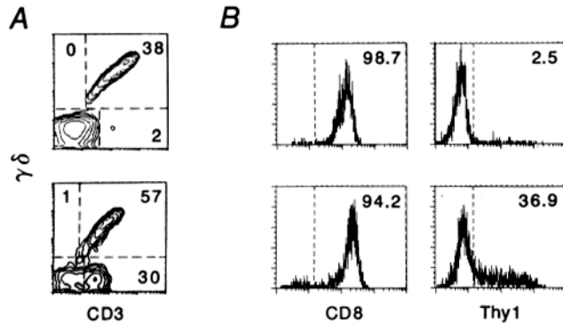
by nu/nu (top) and nu/+ (bottom) \gamma/\delta + IEL. IEL were stained with 3A10 mAb (biotinylated, streptavidin-phycoerythrin) and either Thy-1.2 or CD8 (FITC-conjugated) mAbs. For the Thy-1 and CD8 fluorescence histograms, only 3A10 + cells are shown.
